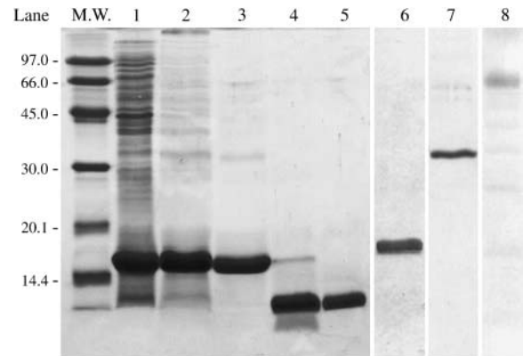
FIGURE 2 Overproduction and purification of human monomeric and polymeric ubiquitins as analyzed by SDS-PAGE. SDS-PAGE analysis of monomeric (lanes 1–5), dimeric (lane 6), tetrameric (lane 7), and octameric (lane 8) ubiquitins was shown. The descriptions of individual lanes are as follows. Molecular weight marker proteins ( M. W. ), total cell lysate of E. coli . BL21(DE3) carry pETUBI 1 after induction (lane 1), the fusion proteins bound to Ni-NTA agarose column (lane 2), the fusion proteins eluted from Ni-NTA agarose column by use of elution buffer containing 40 mM imidazole (lane 3), the eluted fusion proteins after enterokinase cleavage (lane 4), the purified recombinant ubiquitin after removing the His-containing tag region by Ni-NTA affinity chromatography (lane 5), purified dimeric (lane 6), tetrameric (lane 7), and octameric (lane 8) ubiquitins. Recombinant human ubiquitin polymers were purified from E. coli lysate as described under Materials and Methods. Lanes 6, 7, and 8 were cut from separate gels with the positions of the bands adjusted to the markers on the left.
