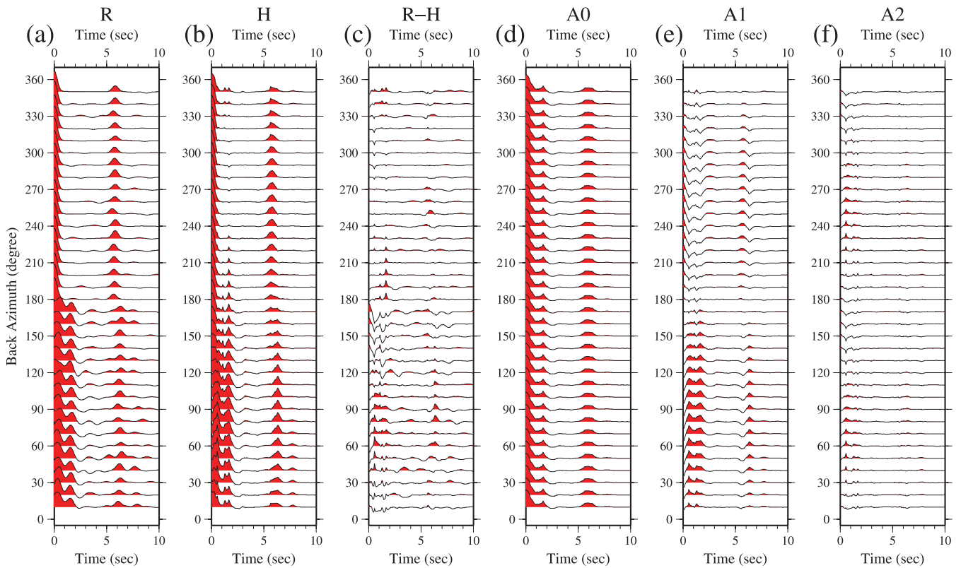
Figure A6. The same as Fig. A3, but for synthetic receiver functions from a model with a 2 km jump of sedimentary layer thickness such that there are no sediments east of the station and 2 km of sediments west of the station.
